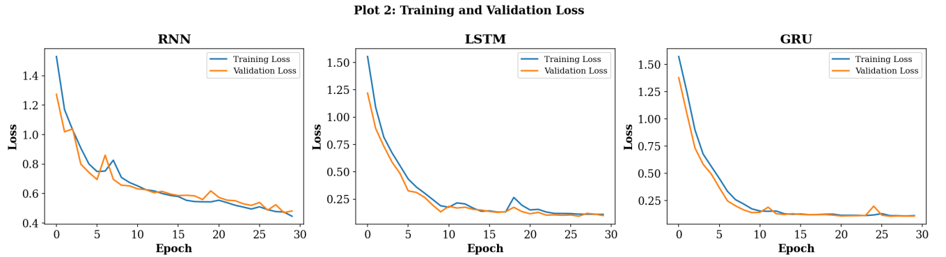
Figure 2: Training and validation loss curves for RNN, LSTM and GRU over 30 epochs.
