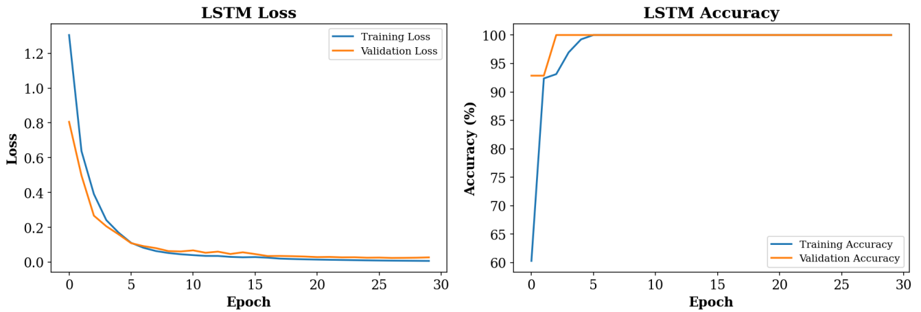
Figure 8: Training and validation loss and accuracy for the CNN–LSTM video classifier over 30 epochs.
