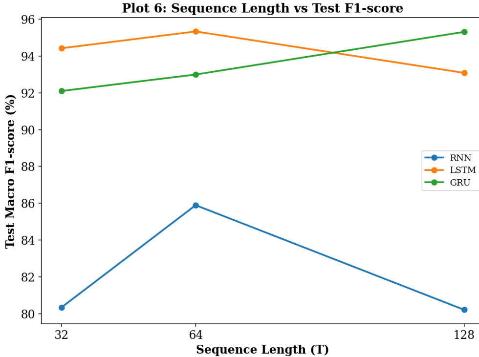
Figure 6: Test macro F1-score against sequence length for RNN, LSTM and GRU.
