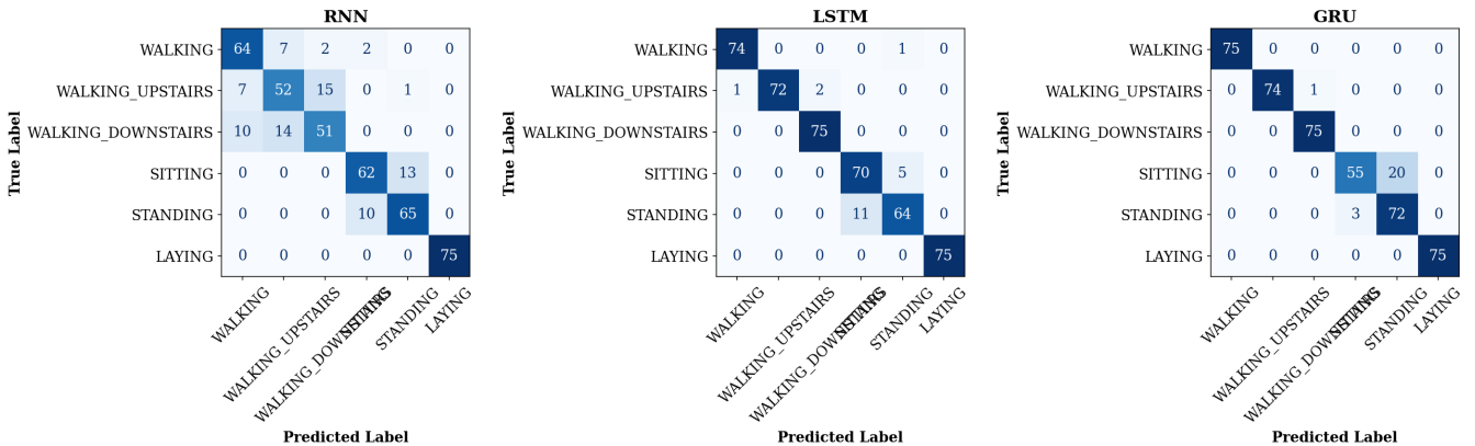
Plot 4: Confusion Matrices (RNN, LSTM, GRU)
