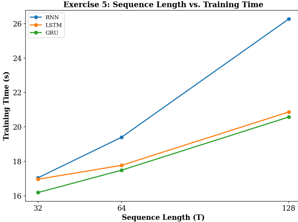
Figure 10: Training time against sequence length for RNN, LSTM and GRU.
