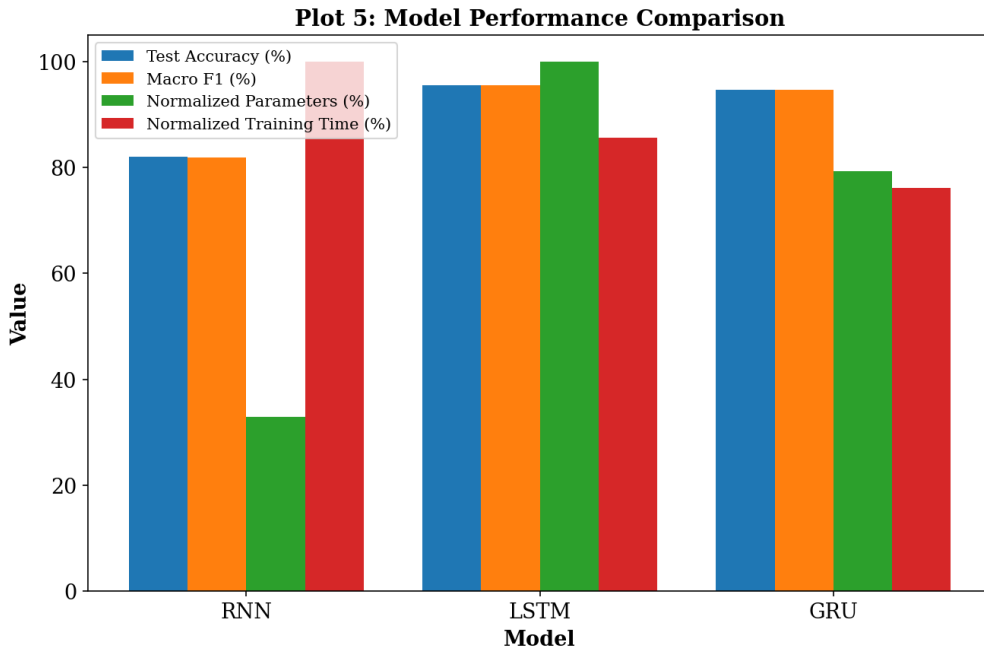
Figure 5: Bar plot comparing test accuracy, macro F1-score, and normalized parameter count and training time for RNN, LSTM and GRU.
