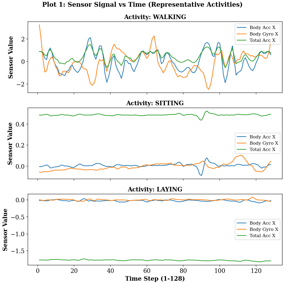
Figure 1: Sensor signal vs. time for Body Acc X, Body Gyro X and Total Acc X, shown for WALKING, SITTING and LAYING.
