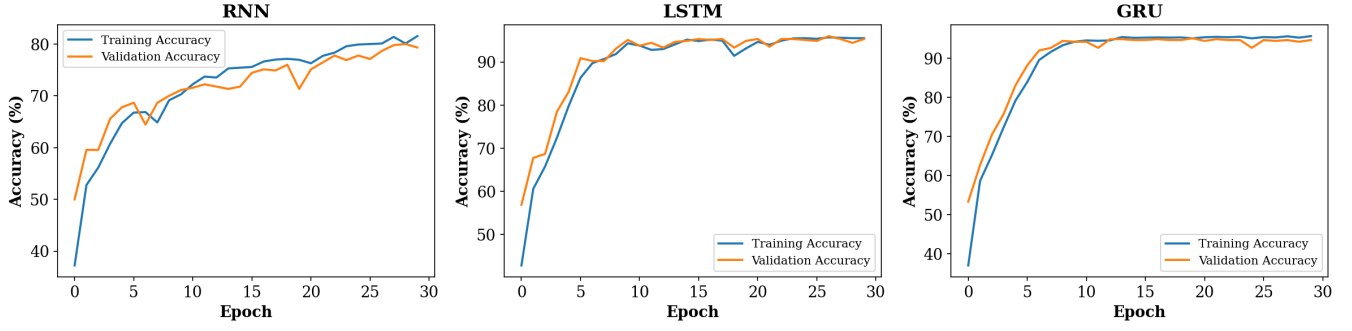
Figure 3: Training and validation accuracy curves for RNN, LSTM and GRU over 30 epochs.
