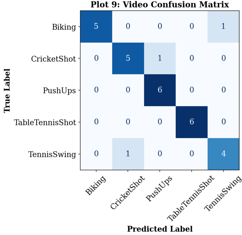
Figure 9: Confusion matrix for the CNN-LSTM video classifier on the test set.
